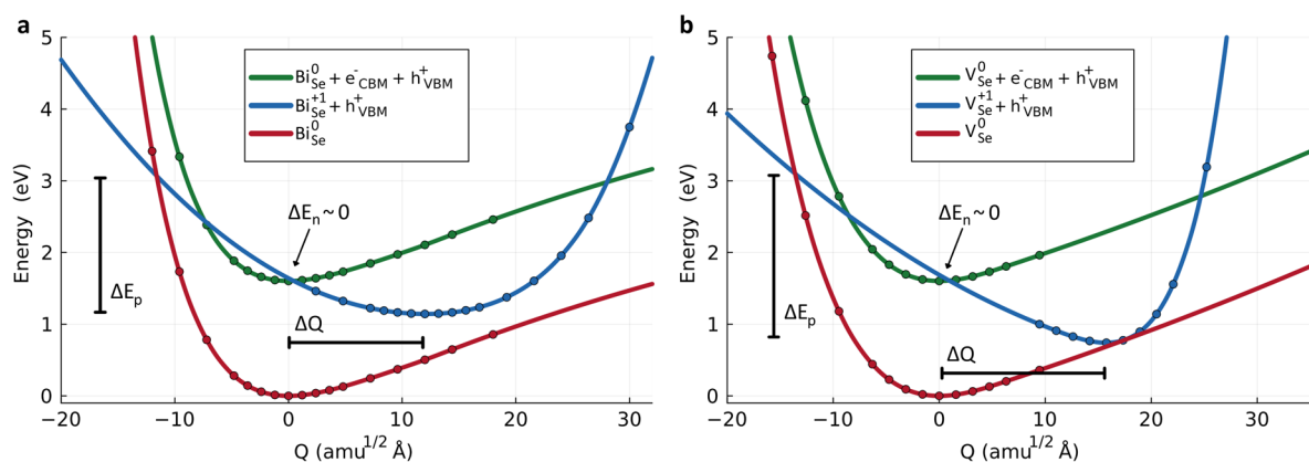
Figure 3. Configuration coordinate diagrams for BiSeI. Configuration coordinate diagrams for a. Bi Se (0/+1) and b. V Se (0/+1). The dots represent potential energies computed from first-principles, and the solid lines are their corresponding quadratic spline interpolation and extrapolation. \Delta Q represents the generalized distance between charge states and \Delta E_x the electron (n)/hole (p) energy capture barriers.
