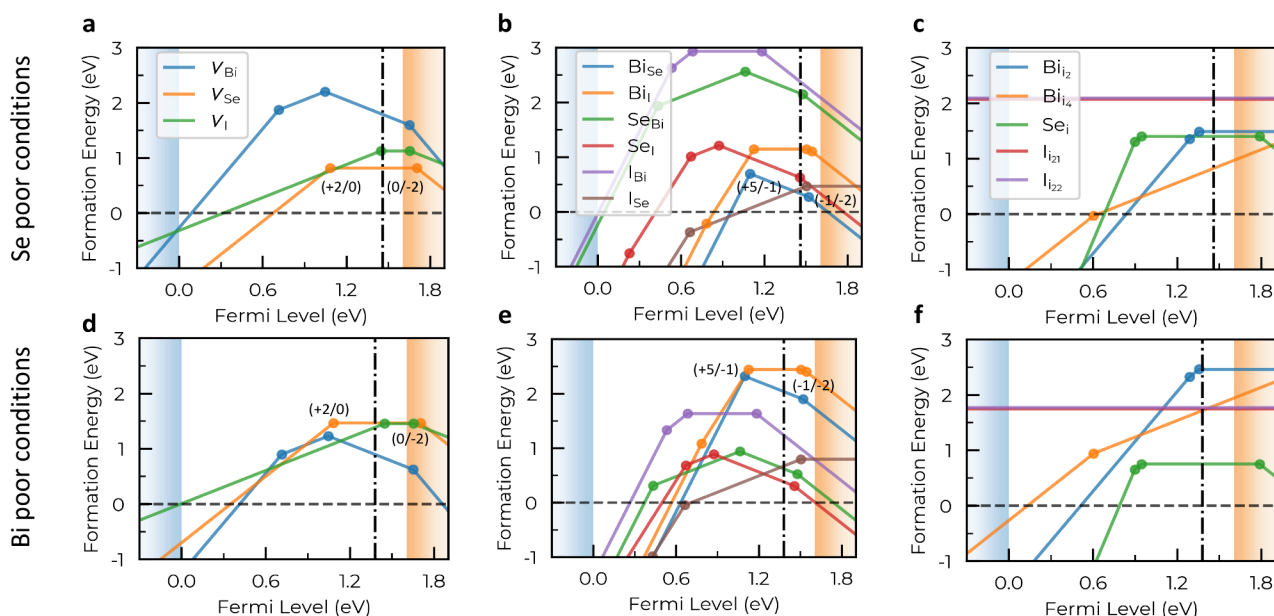
Figure 2. Formation energies of point defects in BiSeI. a–c. Se-poor growth conditions. d–f. Bi-poor growth conditions. The self-consistent Fermi level, E_F^{\text{sc}} , is represented with vertical dash-dot lines, lying at 1.46 and 1.38 eV above the VBM (blue shaded region) for Se-poor and Bi-poor growth conditions, respectively (the CBM is represented by the orange shaded region). Numerical subscripts in panels c and f indicate inequivalent lattice interstitial positions (Supplementary Figure 1).
