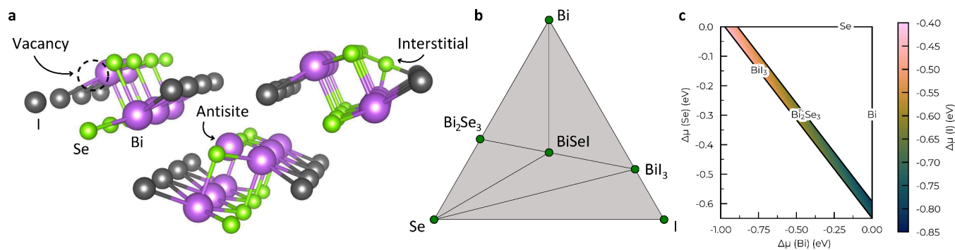
Figure 1. Structural and phase stability properties of BiSeI. a. BiSeI crystal structure (orthorhombic, Pnma ) characterized by columnar motifs held together by weak van der Waals forces. Point defects considered in this study: vacancies, antisites, and interstitials. Bi, Se and I atoms are represented with purple, green and gray spheres, respectively. b. Convex-hull surface of BiSeI calculated with DFT methods. BiSeI is predicted to be thermodynamically stable against separation into secondary phases because its formation enthalpy is negative relative to the convex-hull surface. c. Chemical stability region, delimited by Se-poor ( \mu_{\text{Bi}}, \mu_{\text{Se}}, \mu_{\text{I}} = (0, -0.65, -0.75) eV) and Bi-poor conditions ( \mu_{\text{Bi}}, \mu_{\text{Se}}, \mu_{\text{I}} = (-0.97, 0, -0.42) eV) (Supplementary Table 1).
